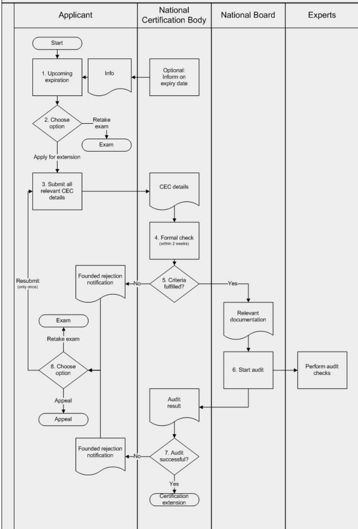
Fig.1 Workflow
